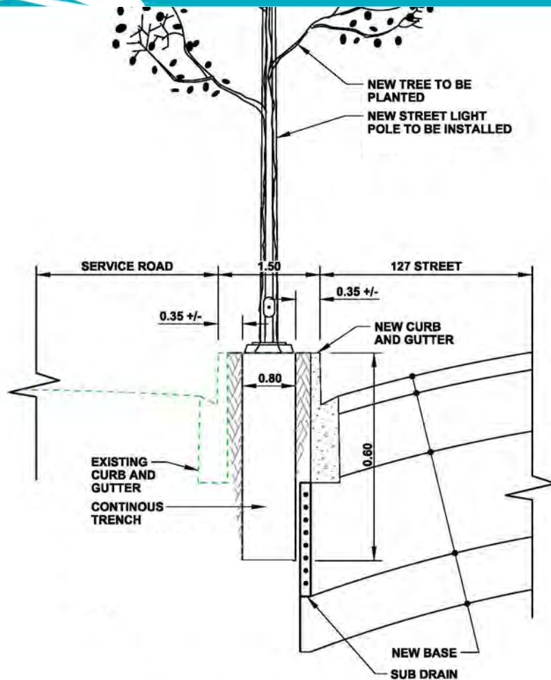
WEST MEDIAN CONTINUOUS SOIL TRENCH (TYPICAL DETAIL)
