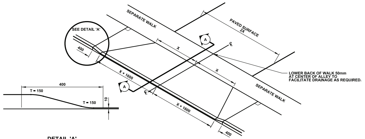
DETAIL 'A'
