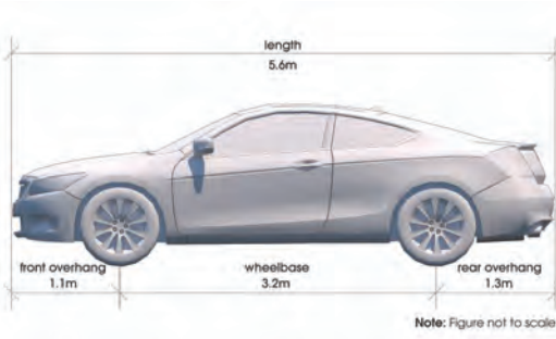
Figure 3.5 Passenger Car Dimensions
