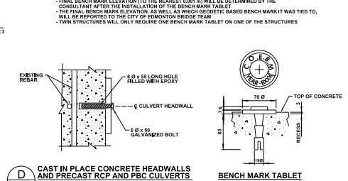
CAST IN PLACE CONCRETE HEADWALLS AND PRECAST RCP AND PVC CULVERTS (CSP SHOWN, PRECAST SIMILAR) 1.3
