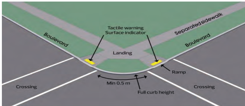
Figure 3.52 Perpendicular Curb Ramps Boulevard Separated Sidewalk
