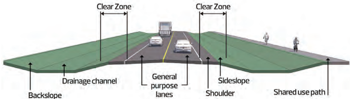
Figure 3.42 Non-Urban Roadside Areas
