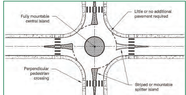
Figure 3.71: Features of a Typical Mini-Roundabout (Source: TAC Canadian Roundabout Design Guide Figure 9.21.1)
