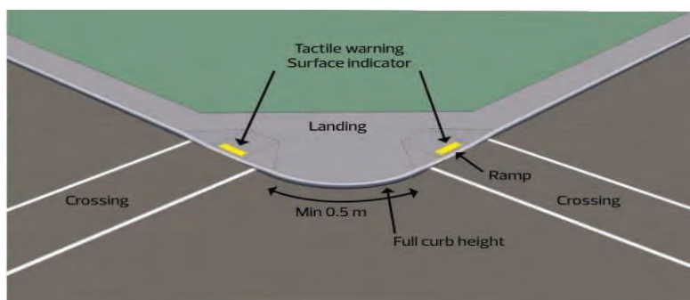
Figure 3.53 Perpendicular Curb Ramps Monolithic Sidewalk
