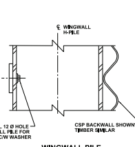
WINGWALL PILE 1.3
