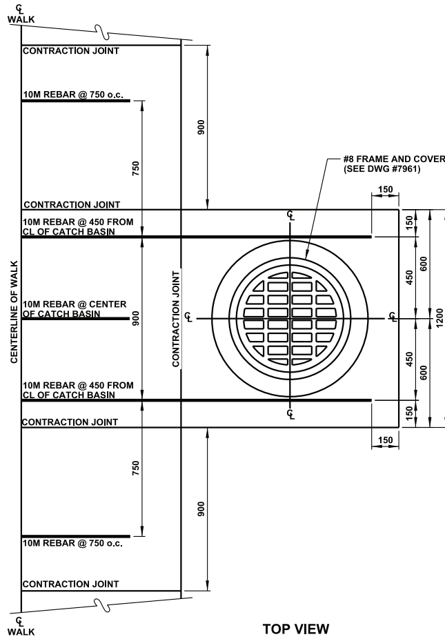
TOP VIEW
