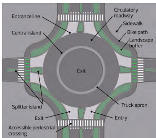
Figure 3.70: Basic Geometric Design Features of a Roundabout
