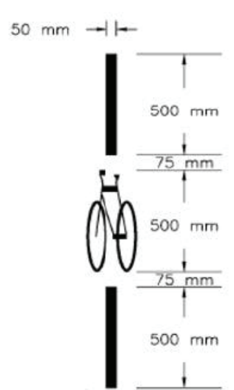
Figure 3.82 Bicycle Detection Marking Symbol (Source: TAC Bikeway Traffic Control Guidelines for Canada, Section 7.4.6, Figure 3.4)
