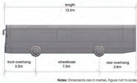
Figure 3.7 B-12 Standard Single Unit Bus Dimensions
