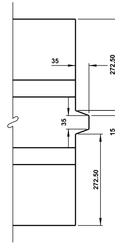
DETAIL 'A'
