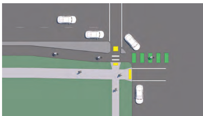
Figure 3.61: Protected Bicycle Signal Phase with Bend-Out
