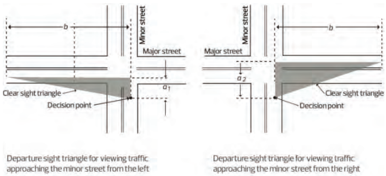
Figure 3.48 Departure Sight Triangles (Stop-Controlled) (Adapted from TAC GDG Figure 9.9.2)
