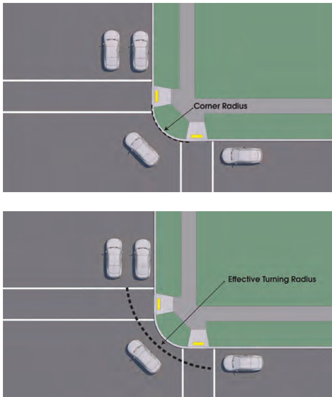
Figure 3.49 Corner Radii and Effective Turn Radius
