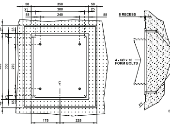
INSTALLATION DETAILS LARGE PLAQUE 1.3
