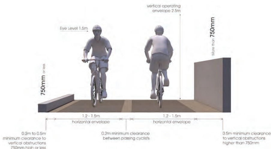
Figure 3.4 Bicycle Operating Space
