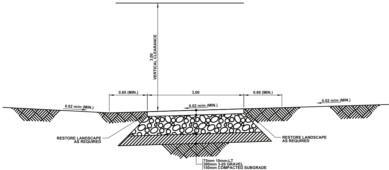
TYPICAL SECTION
