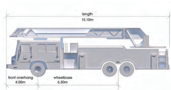
Figure 3.8 City of Edmonton Fire Truck Dimensions
