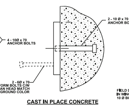
CAST IN PLACE CONCRETE 1.3
