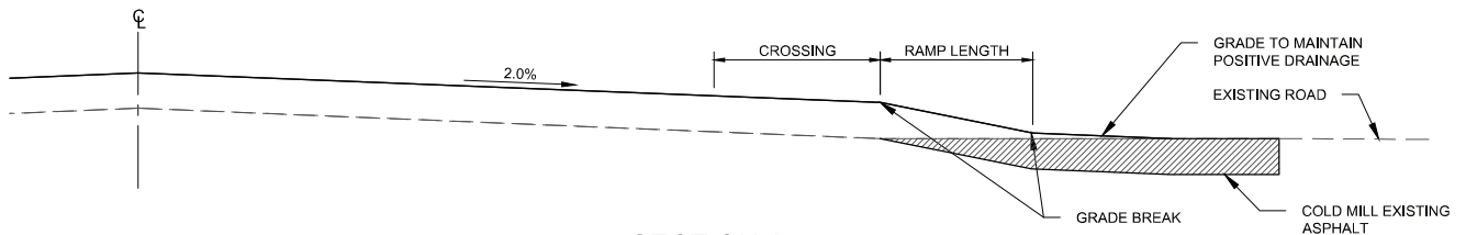
SECTION A
