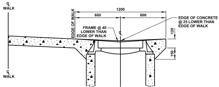
CROSS-SECTION VIEW
