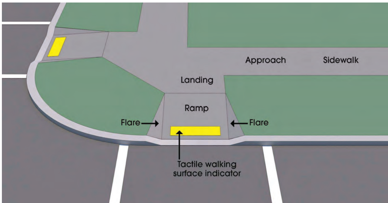
Figure 3.51 Parts of the Curb Ramp
