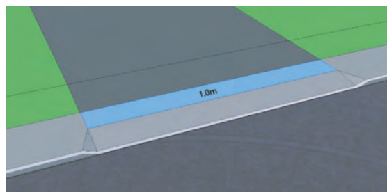
Figure 3.40B: Driveway crossing of monolithic walk
