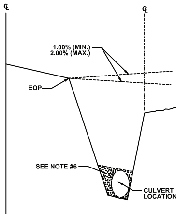
SECTION B-B
