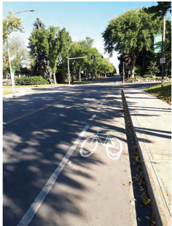
Figure 3.64: Bike Lane Intersection Treatments without Right Turn Lane
