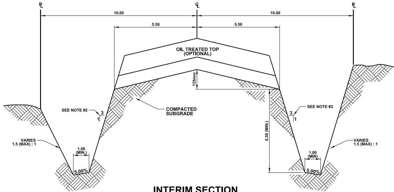
INTERIM SECTION
