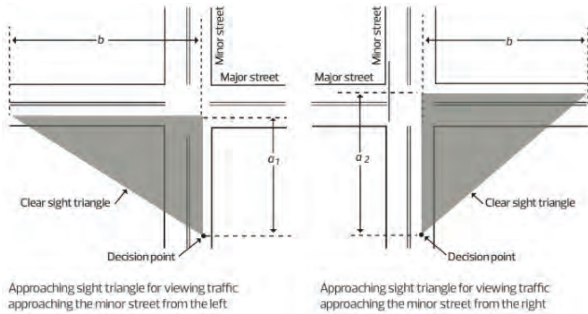
Figure 3.47 Approach Sight Triangle (Yield-Controlled) (Adapted from TAC GDG Figure 9.9.1)
