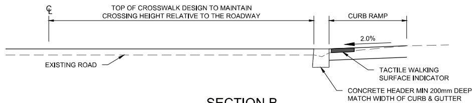
SECTION B
