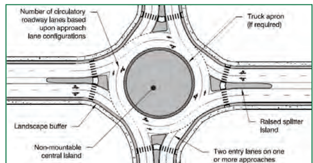
Figure 3.73: Features of a Typical Multi-Lane Roundabout (Source: TAC Canadian Roundabout Design Guide Figure 9.21.3)
