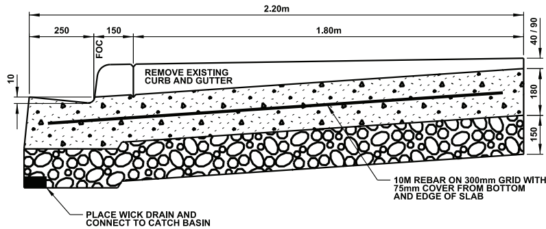
SECTION A-A STRAIGHT FACE
