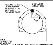
CAST IN PLACE CONCRETE HEADWALLS AND PRECAST CULVERTS (CSP SHOWN, PRECAST SIMILAR) N.T.S.
