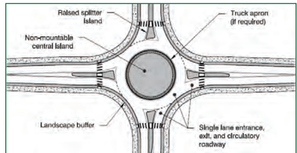
Figure 3.72: Features of a Typical Single-Lane Roundabout (Source: TAC Canadian Roundabout Design Guide Figure 9.21.2)
