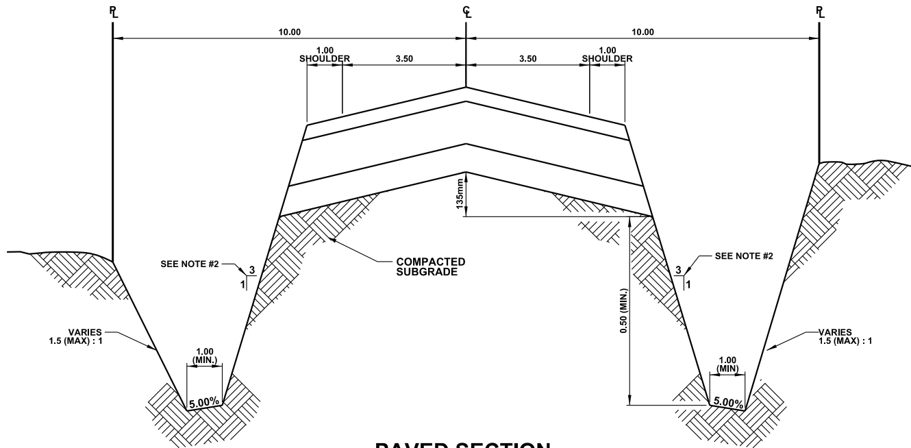
PAVED SECTION
