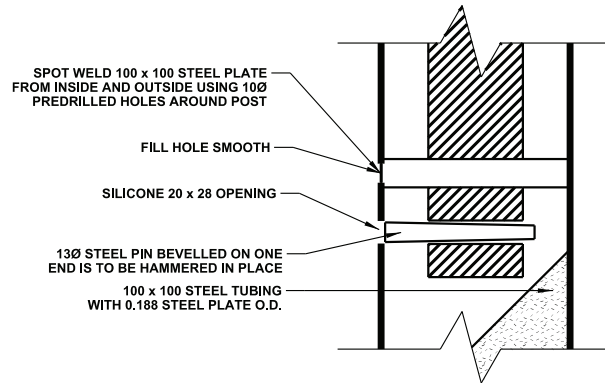
ASSEMBLY DETAIL
