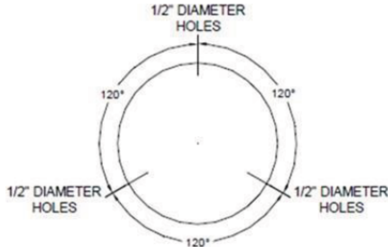
Figure 4: Recommended Pipe Perforations
