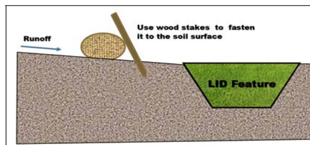
Figure 8: Fibre Roll Installation
