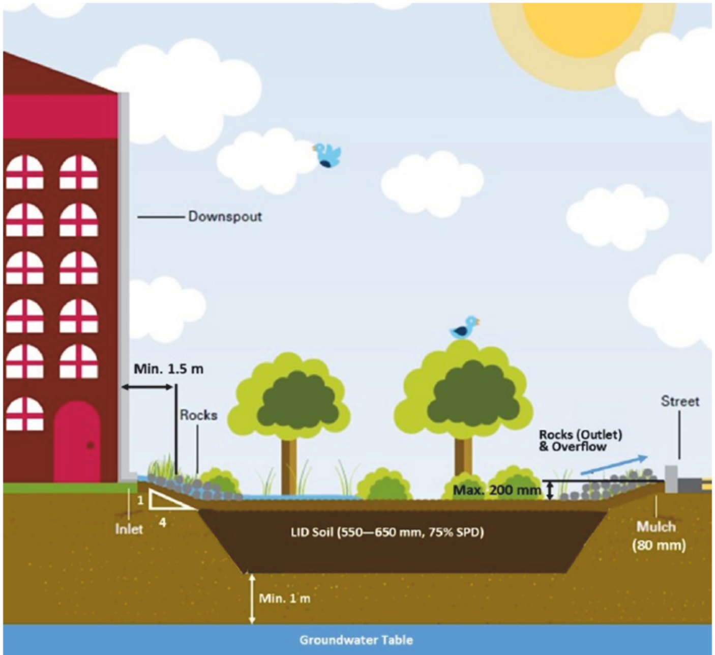
Figure 3: Rain Garden Profile
