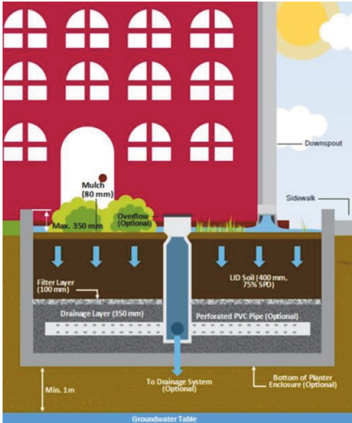
Figure 6: Box Planter Section
