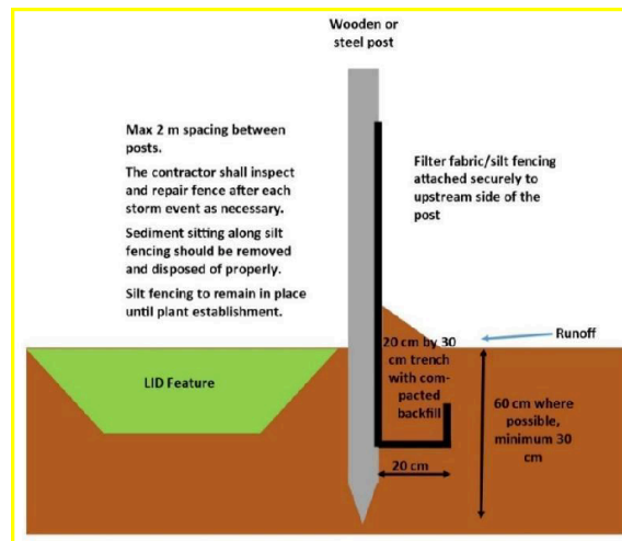
Figure 7: Silt Fence Installation
